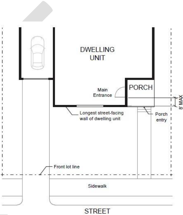
Figure for 8.120.C.4.b.iv Main Entrance Opening onto a Porch
